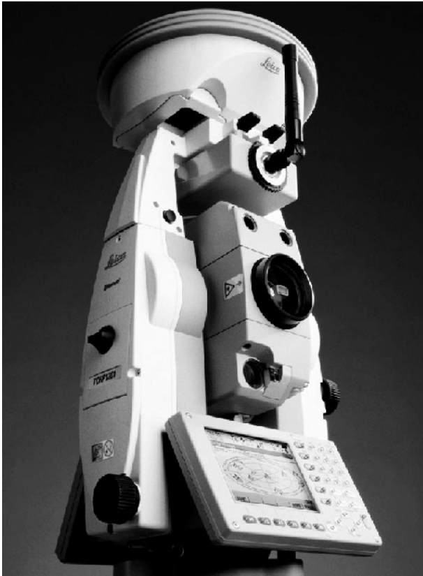
Figure 3 – SmartStation
